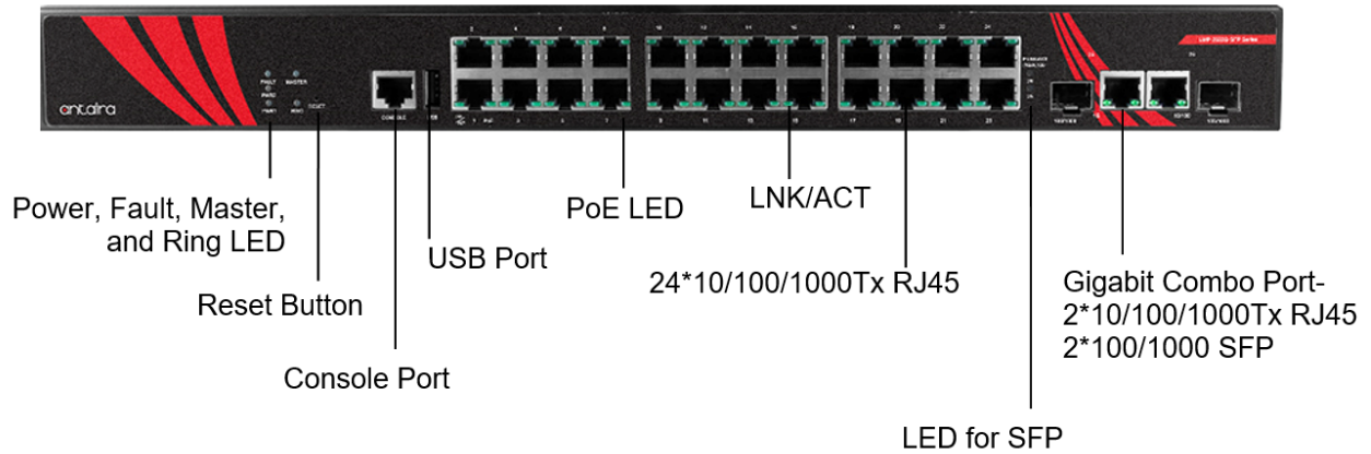
Figure 2.2 - Front View Panel
