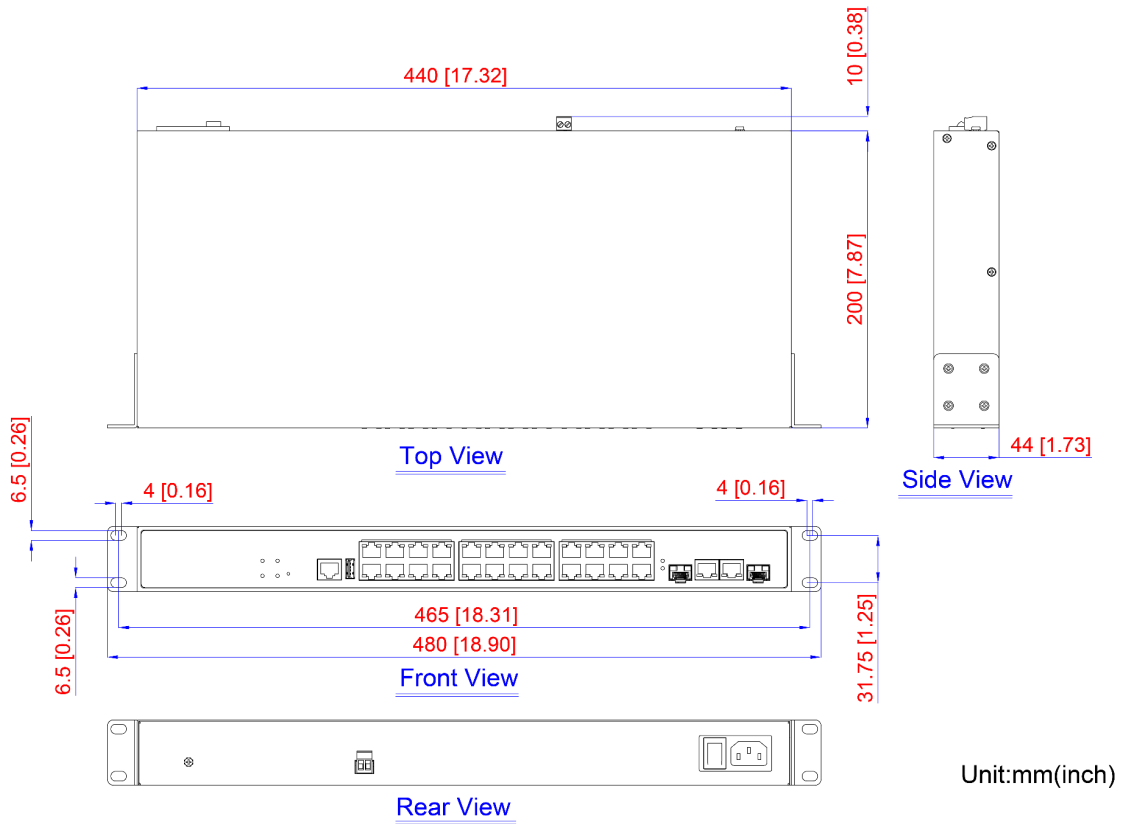
Figure 2.1 - Physical Dimensions
